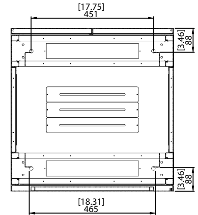
CUT-OPEN
